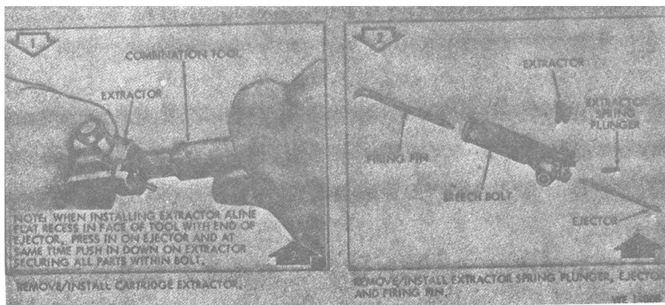
Figure 2-6. Remove/install cartridge extractor and components .
